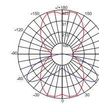
Luminous Intensity Unit : cd/klm Lens Code : S1S113 Type I
