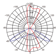
Luminous Intensity Unit : cd/klm Lens Code : A2S111 Type II
